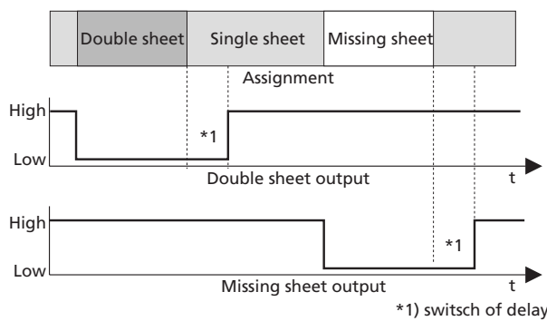
Fig. 8: dbk-5/CDD/O/M30 time diagram Free-Run-Mode
