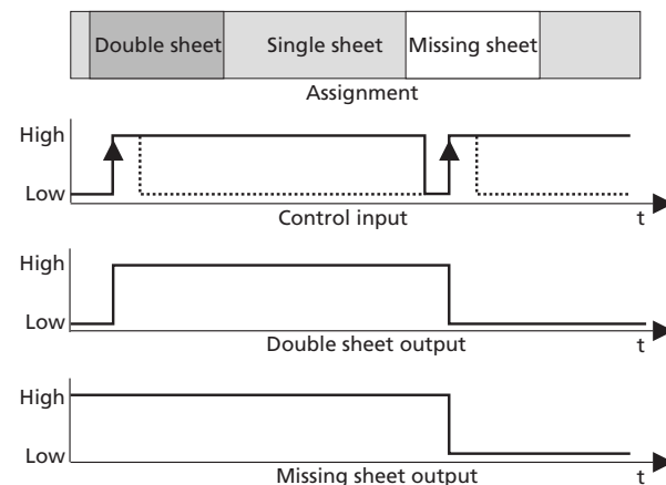
Fig. 10: dbk-5/BDD/O/M30 time diagram Trigger-Mode
