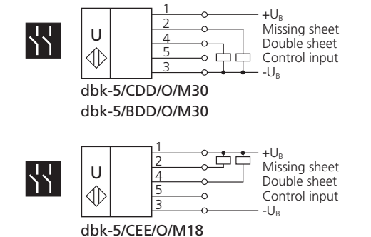
Fig. 2: Standard symbols and terminal assignment
