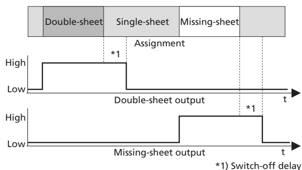
Fig. 9: dbk-5/CEE/O/M30 time diagram Free-Run-Mode
