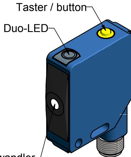
Ultraschallwandler ultrasound transducer
