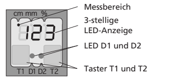
Abb. 3: TouchControl
