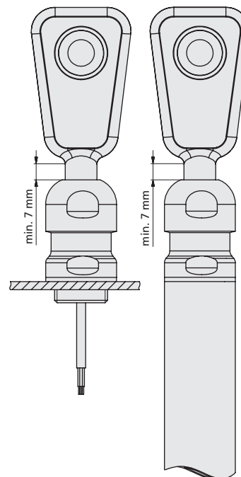
Fig. 6: pms sensor D12 adapter shaft with sensor screw connection BF-pms/A1 mounted to machine part or to stainless steel tube D26.8 with internal thread M20x1.5
