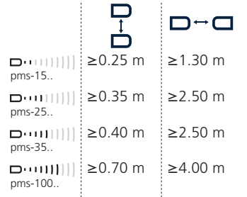
Fig. 2: Assembly distances to avoid a mutual influence of the sensors
