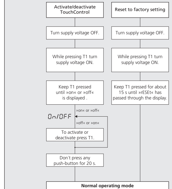
Diagram 3: Key lock and factory setting
