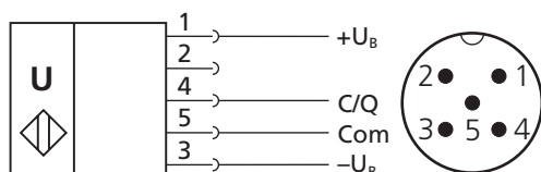
Fig. 3: Connection diagram of the mic+ sensor
