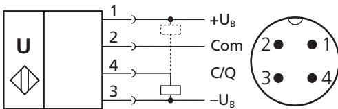
Fig. 3: Connection diagram of the nano sensor
