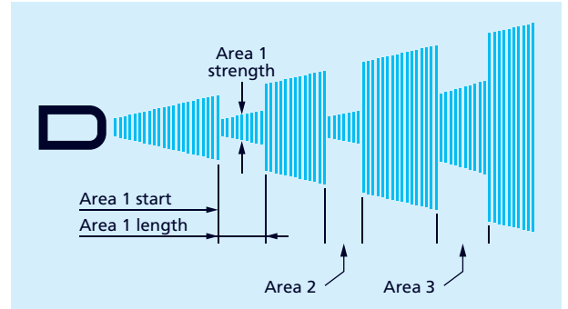
Fig. 14: Setting options for the interference echo suppression
