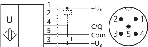
Fig. 3: Connection diagram of the cube sensor
