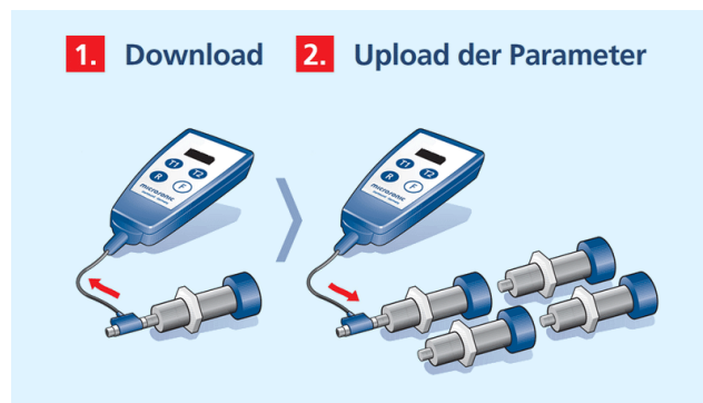
LinkCopy: Copying of sensor settings
