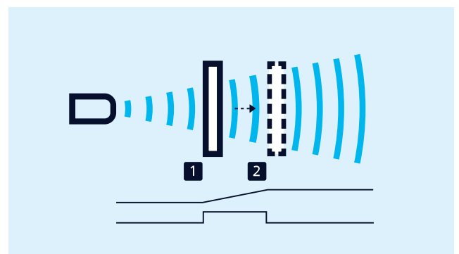
Teach-in of an analogue characteristic or of a window with two switching points
