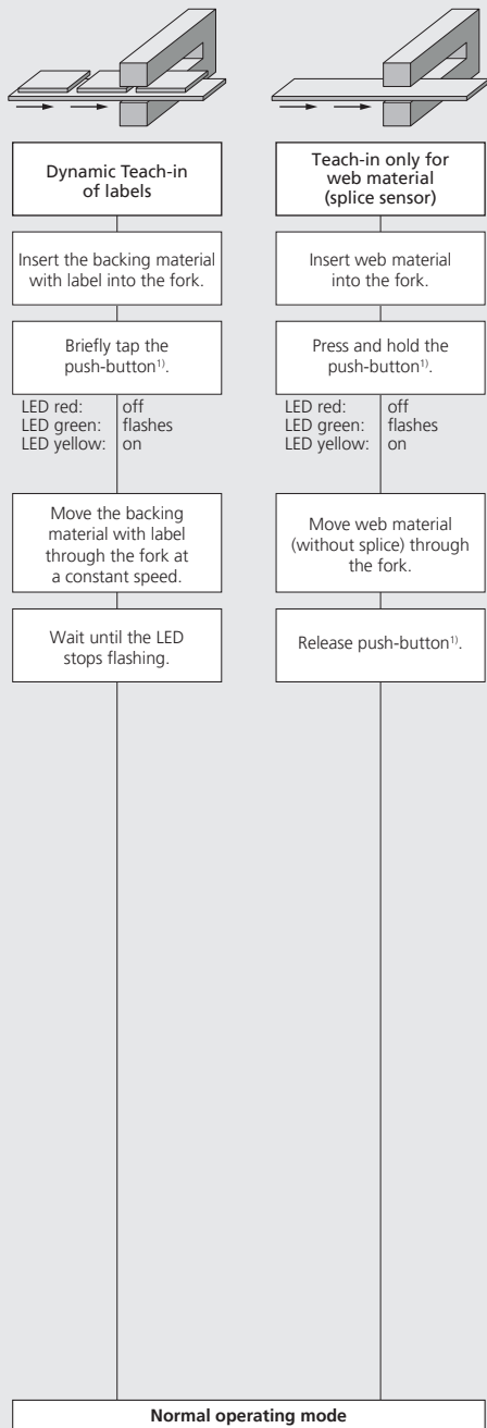
Diagram 1: Standard Teach-in
