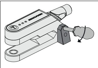
Fig. 6: Removing the mounting adapter
