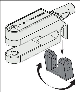
Fig. 5: Adjust the angle by rotating the mounting adapter
